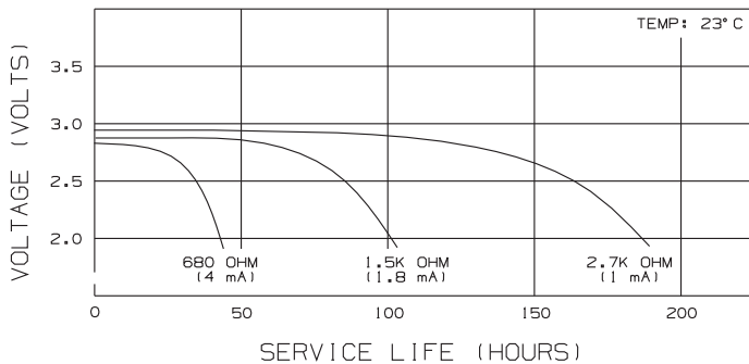
Typical Discharge Characteristics K58L
